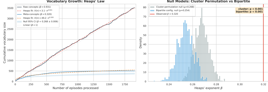
Fig. 3. Left: Heaps’ law vocabulary growth ( \beta = 0.931 raw, 0.320 meta-concept). Right: null model distributions—cluster-permutation ( \beta_{\text{null}} = 0.268 ) and bipartite configuration ( \beta_{\text{null}} = 0.254 ), both p < 0.001 .
