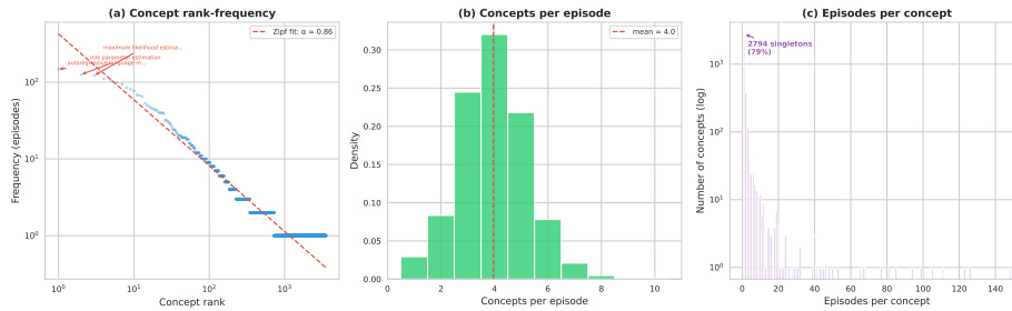
Fig. 1. Concept frequency distributions. Left: Zipf rank-frequency (exponent \approx 0.86 ). Center: concepts per episode (mean 3.96). Right: episodes per concept (79% singletons).
