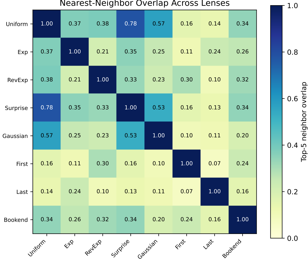
Nearest-Neighbor Overlap Across Lenses
