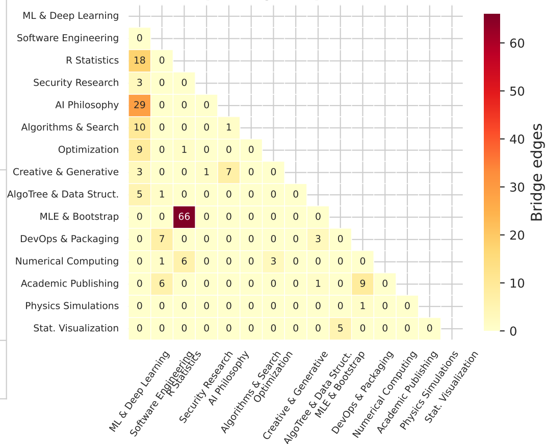
(c) Cross-concept bridges (episodic network, \theta=0.9 )
