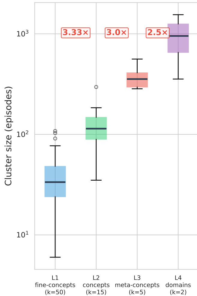
(b) Cluster size distributions
