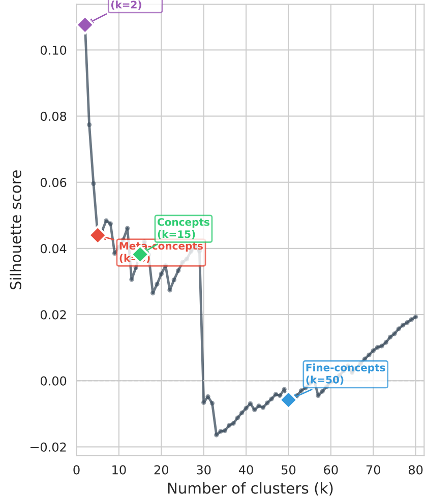
(a) Silhouette score vs. cluster count
