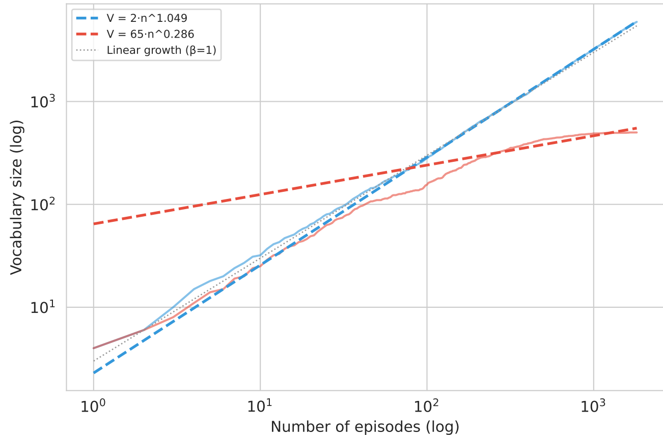
(b) Log-log Heaps' law
