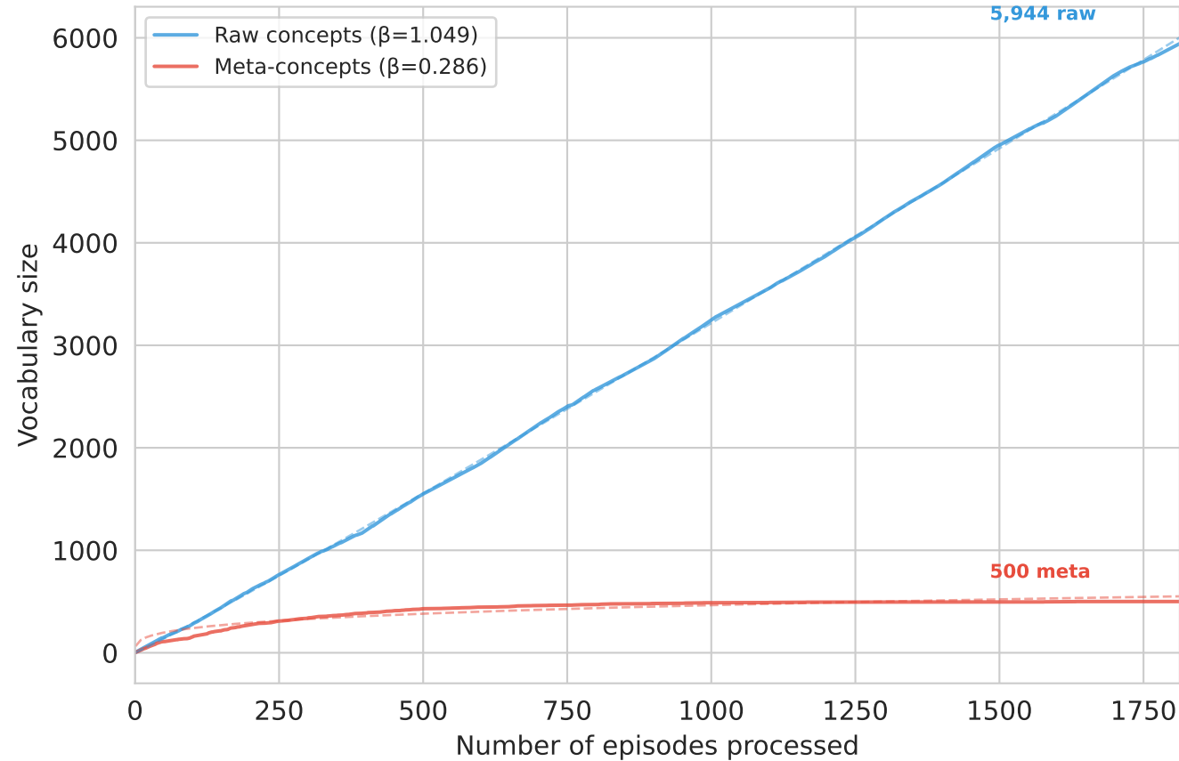
(a) Heaps' law: vocabulary growth
