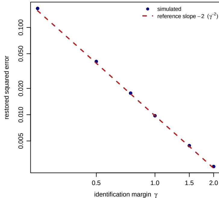
(b) error vs \gamma (slope -2.01 )
