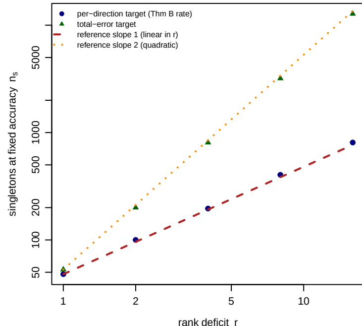
(c) n_s vs r (per-dir 1.02, total 1.98)
