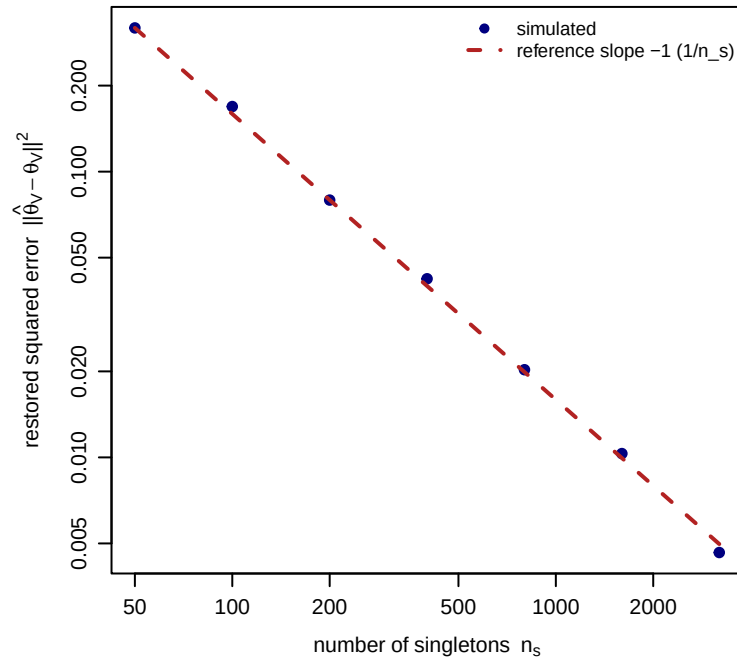
(a) error vs n_s (slope -1.01 )
