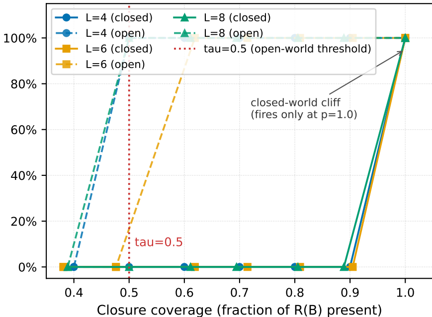
Held-out recovery
