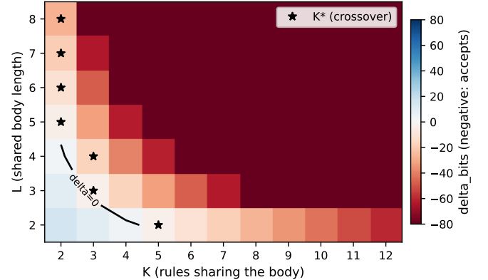
Fig. 1. The abstraction-maturity threshold for body-pattern extraction (EX30). Cell color is the bits-length change of extracting a body shared by K rules of length L : blue where extraction compresses (and the bits gate accepts), red where it does not. The black contour is the break-even ( \Delta = 0 ) line and stars mark the per- L crossover K^* . Clause count accepts every cell ( \Delta = +1 ), blind to the surface.
