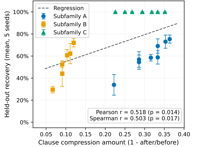
Fig. 2. Compression predicts generalization (EX38). Each point is one of twenty-two synthetic domains; the horizontal axis is the clause compression a symbolic dream achieves (1–ratio), the vertical axis is the mean fraction of held-out generalizations the compressed rules recover, and error bars span five held-out splits. The size-controlled correlation is significant (Pearson r = 0.52 , p = 0.014 ).
