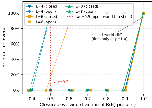
Fig. 3. Open-world recursive discovery closes the partial-closure gap (EX35–37). Fraction of held-out closure pairs recovered as a function of how complete the observed relation is, for three chain lengths. The closed-world exact-match gate (solid) fires only at full completeness; the open-world subset gate (dashed) fires and recovers at every coverage at or above \tau = 0.5 (vertical line), with zero spurious derivations throughout.
