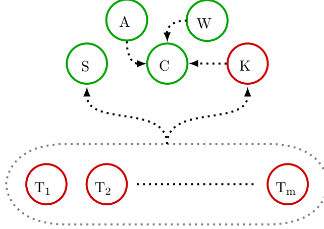
Figure 2: Graphical model of random variables where S = \min\{T_1, T_2, \dots, T_m\} , C is a random \alpha -masked candidate set of cardinality w , K is the random component failure, W is the cardinality of random candidate sets, and A is the random \alpha .
