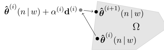
Figure 6: Projection onto convex set \Omega .
