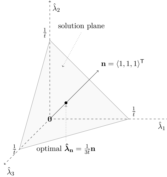
Figure 3: \hat{\lambda}_{\mathbf{n}} solutions given three candidates
