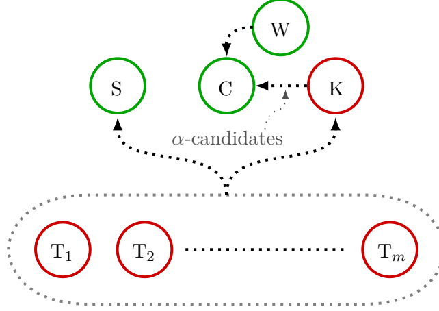
Figure 2: Graphical model of random variables where S = \min\{T_1, T_2, \dots, T_m\} , C is a random \alpha -candidate set, K is the random component failure, and W is the cardinality of random candidate sets.
