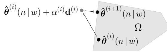
Figure 7: Projection onto convex set \Omega .
