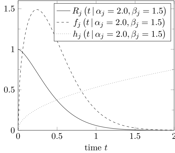
Figure 5: Weibull
