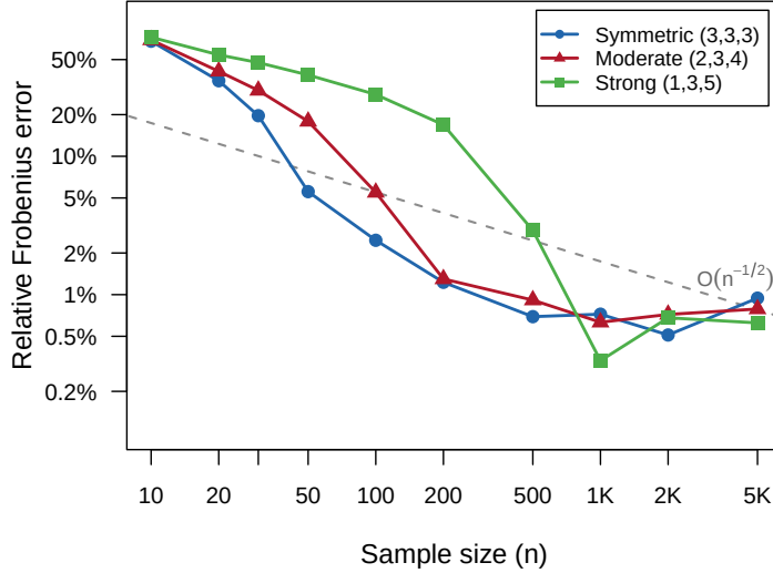
Fig. 1 Relative Frobenius error between the empirical covariance of the MLE and the theoretical asymptotic covariance \frac{1}{n}\mathcal{I}^{-1}(\boldsymbol{\lambda} \mid w=2) , as a function of sample size n ( R = 10^5 replications per point; non-identifiable samples filtered via the triangle inequality (50)). The symmetric and moderate configurations track the O(n^{-1/2}) reference line (dashed); the strongly asymmetric case converges more slowly due to the rarity of candidate sets involving the weakest component.
