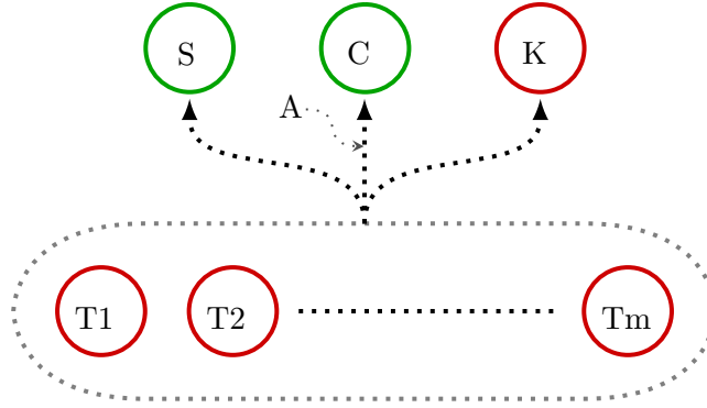
Figure 1: Graphical model of random variables
