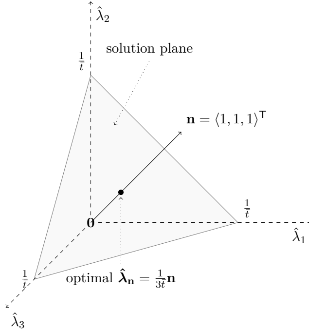
Figure 2: \hat{\lambda}_{\mathbf{n}} solutions given three candidates
