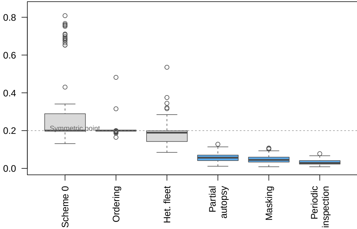
MAE (sorted rates)
