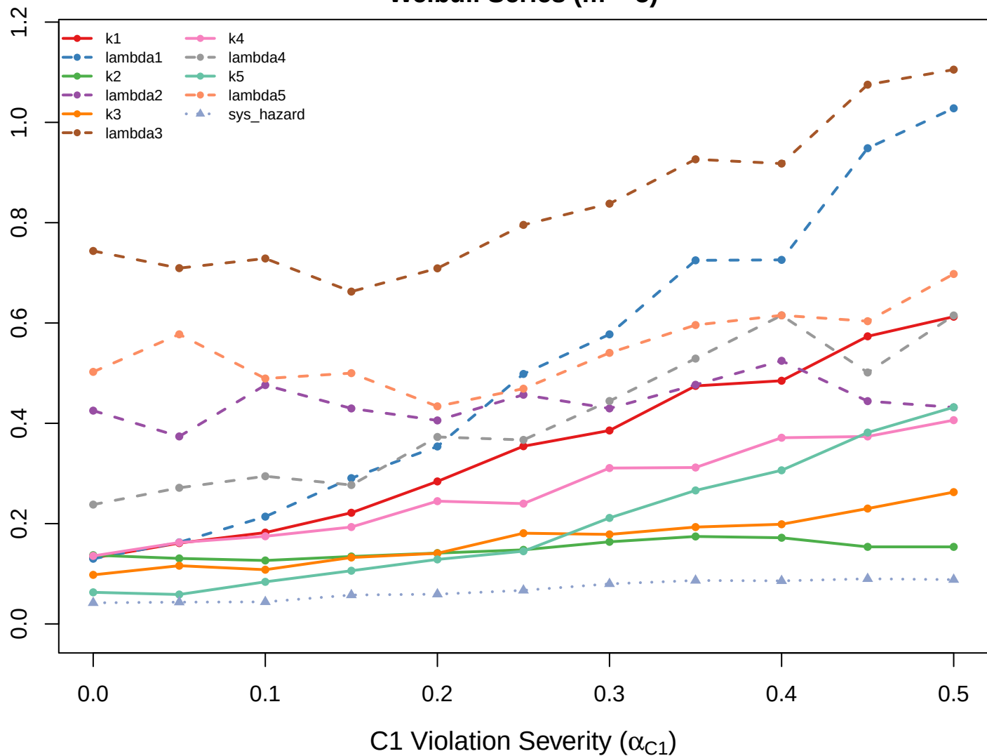
Weibull Series (m = 5)
