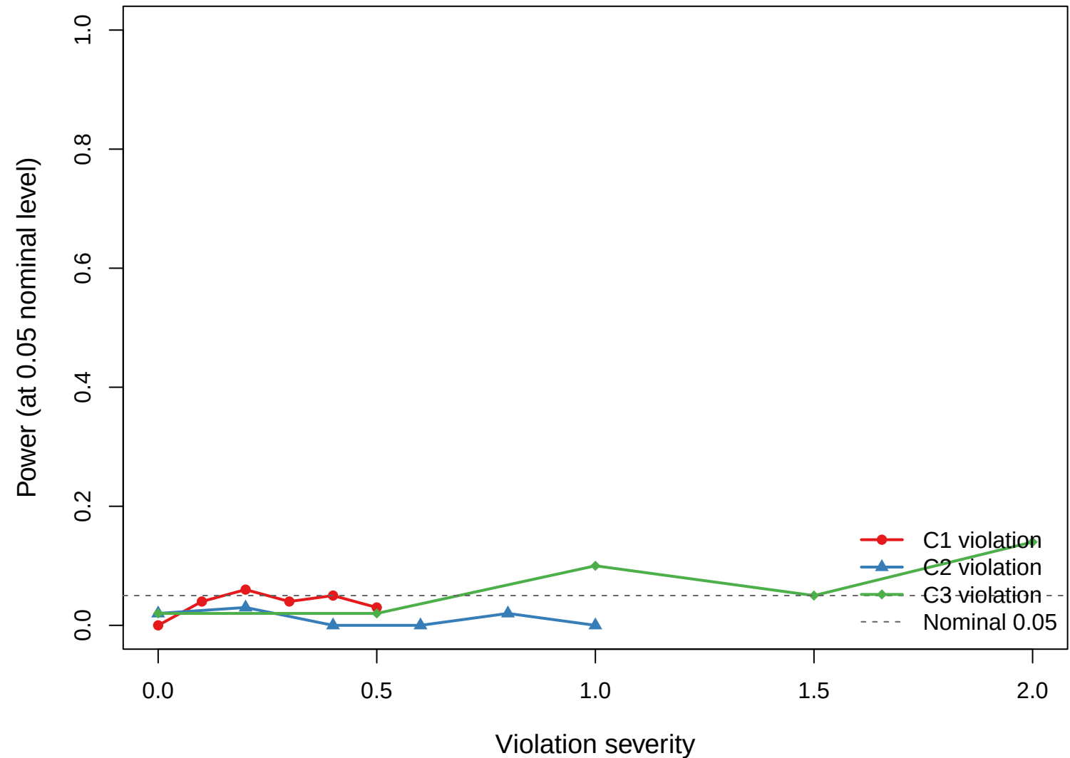
Specification test power
