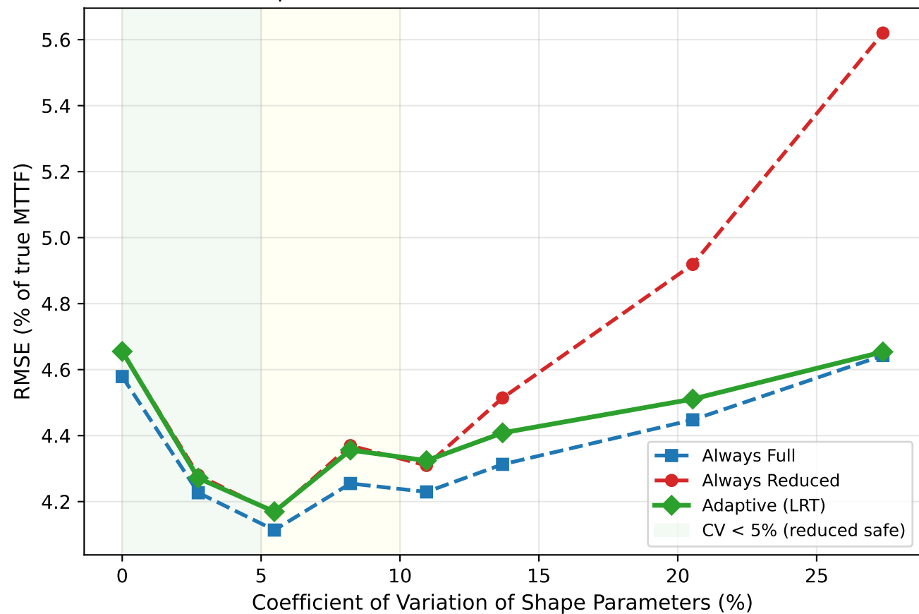
Adaptive Model Selection Performance (n=500)
