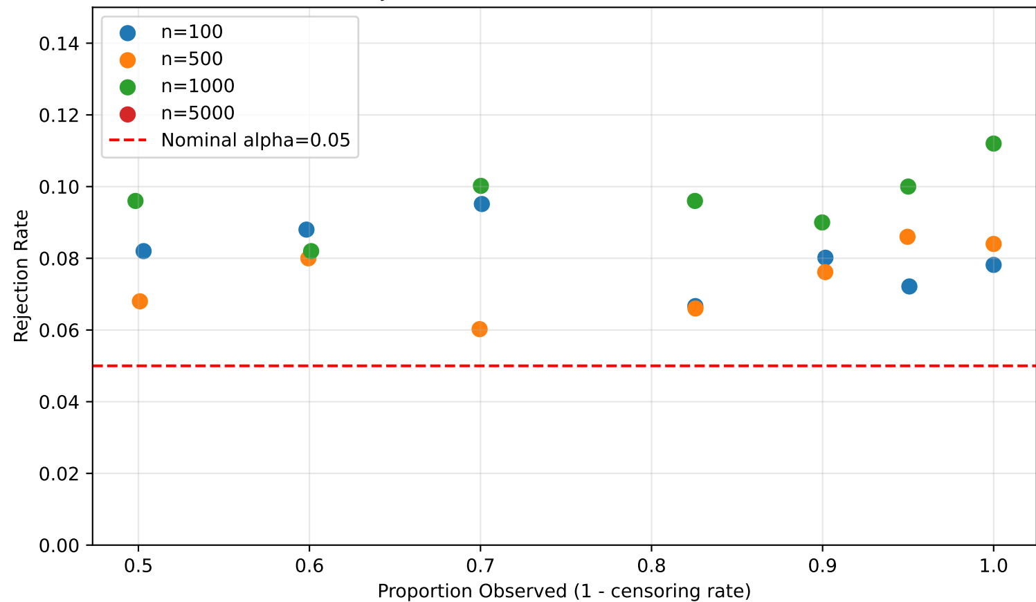
Rejection Rate vs Information Content
