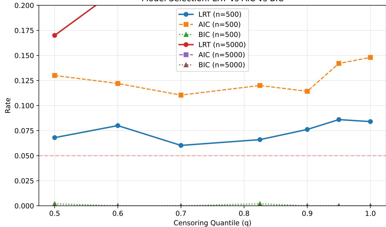
Model Selection: LRT vs AIC vs BIC
