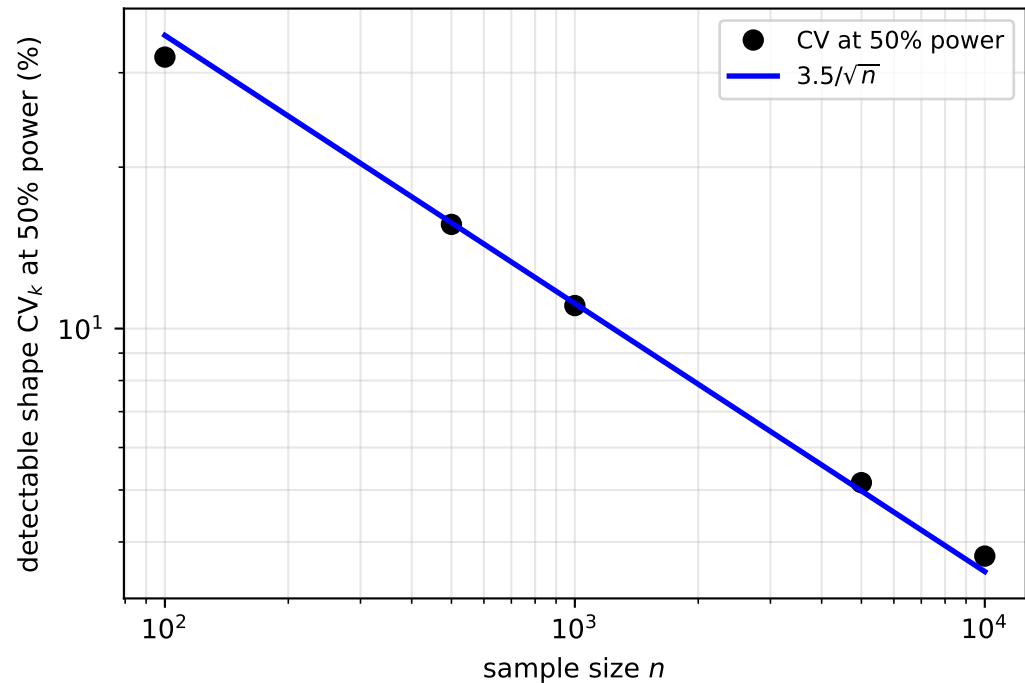
(b) Detection threshold falls as 1/\sqrt{n}
