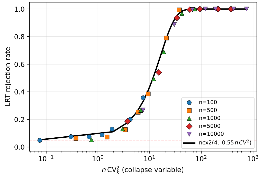
(a) Power collapses onto one noncentral- \chi^2 curve
