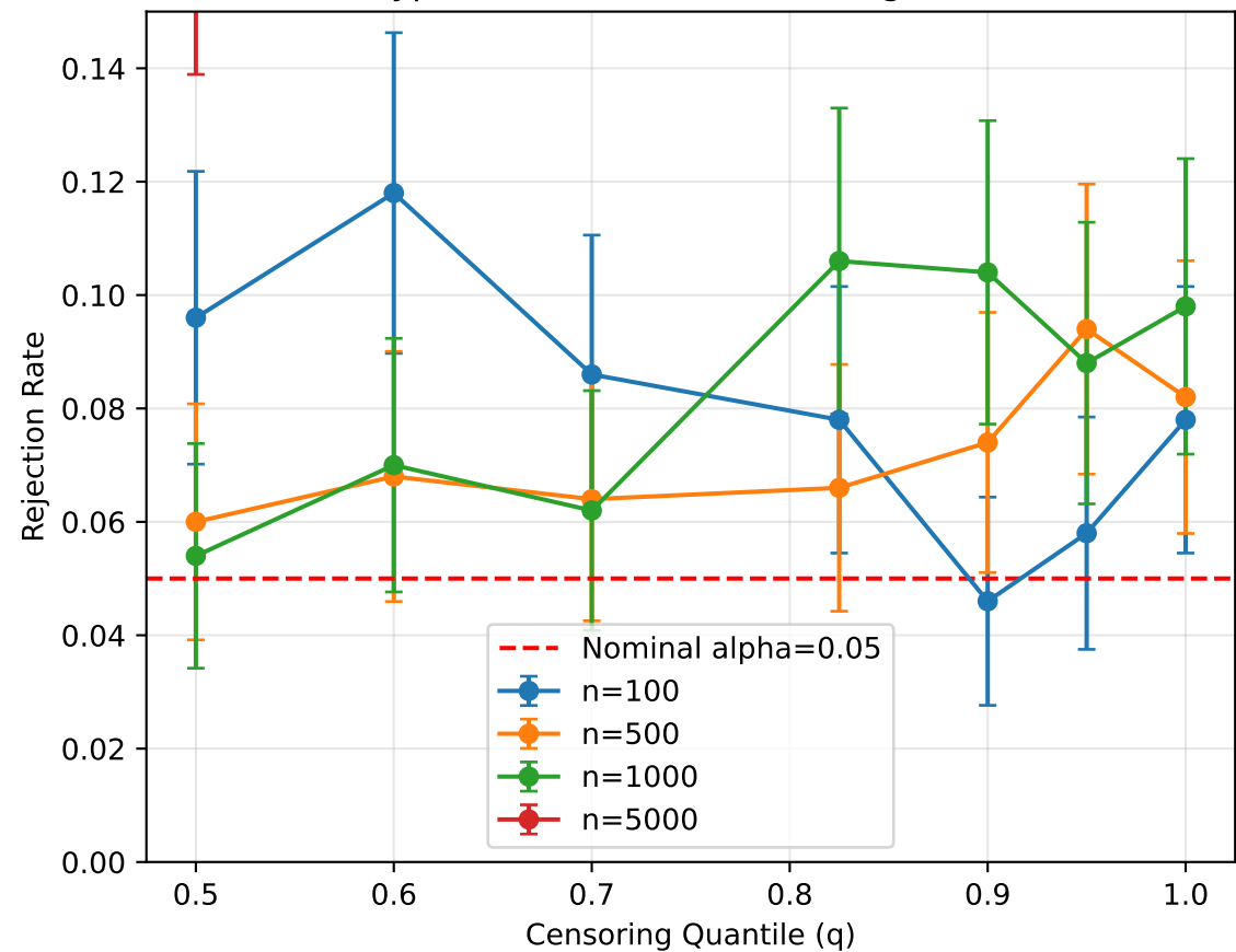
Type I Error Rate vs Censoring Level
