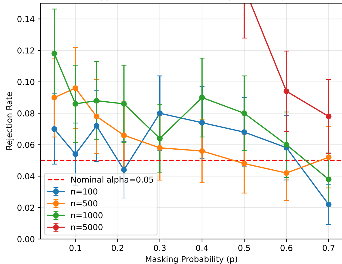
Type I Error Rate vs Masking Probability
