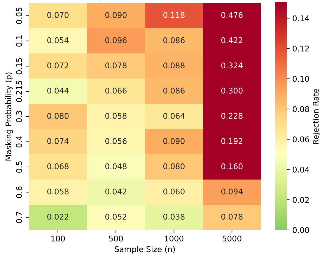
Rejection Rate Heatmap
