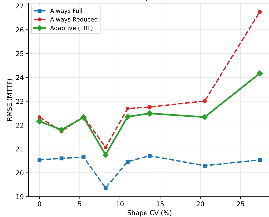
(c) RMSE Comparison (n=100)
