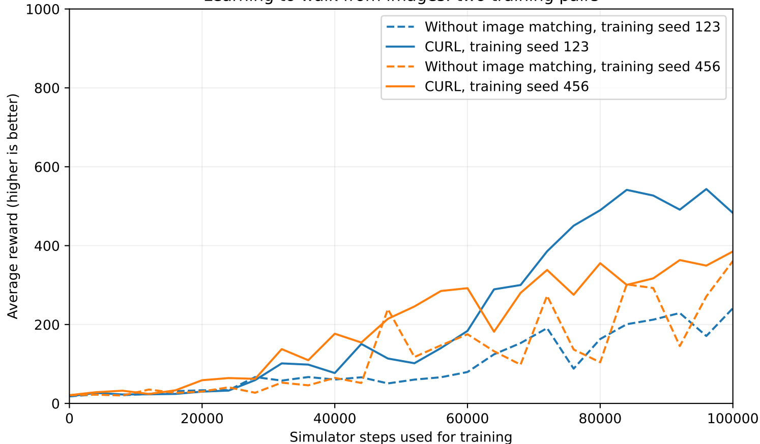
Learning to walk from images: two training pairs
