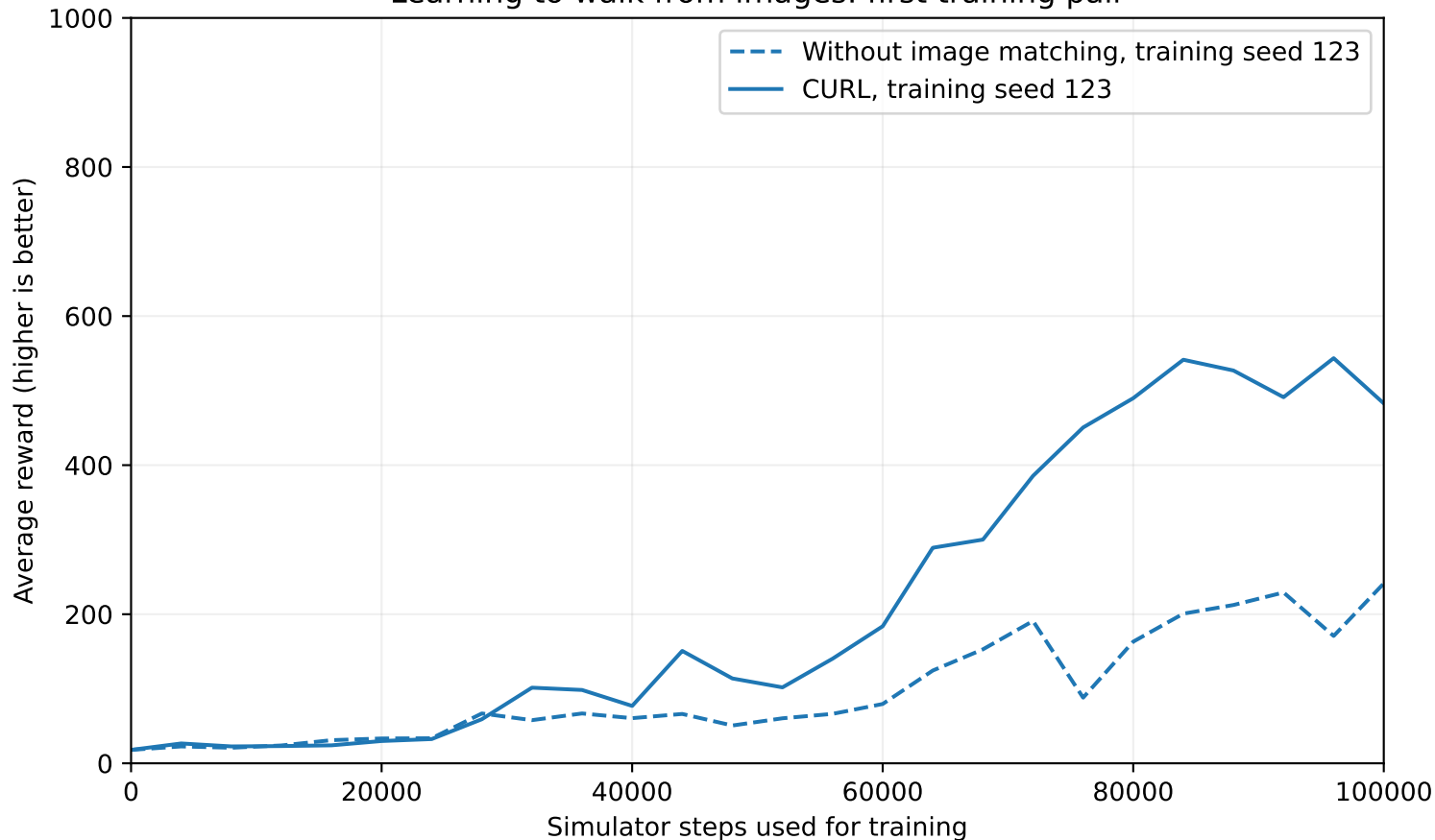
Learning to walk from images: first training pair
