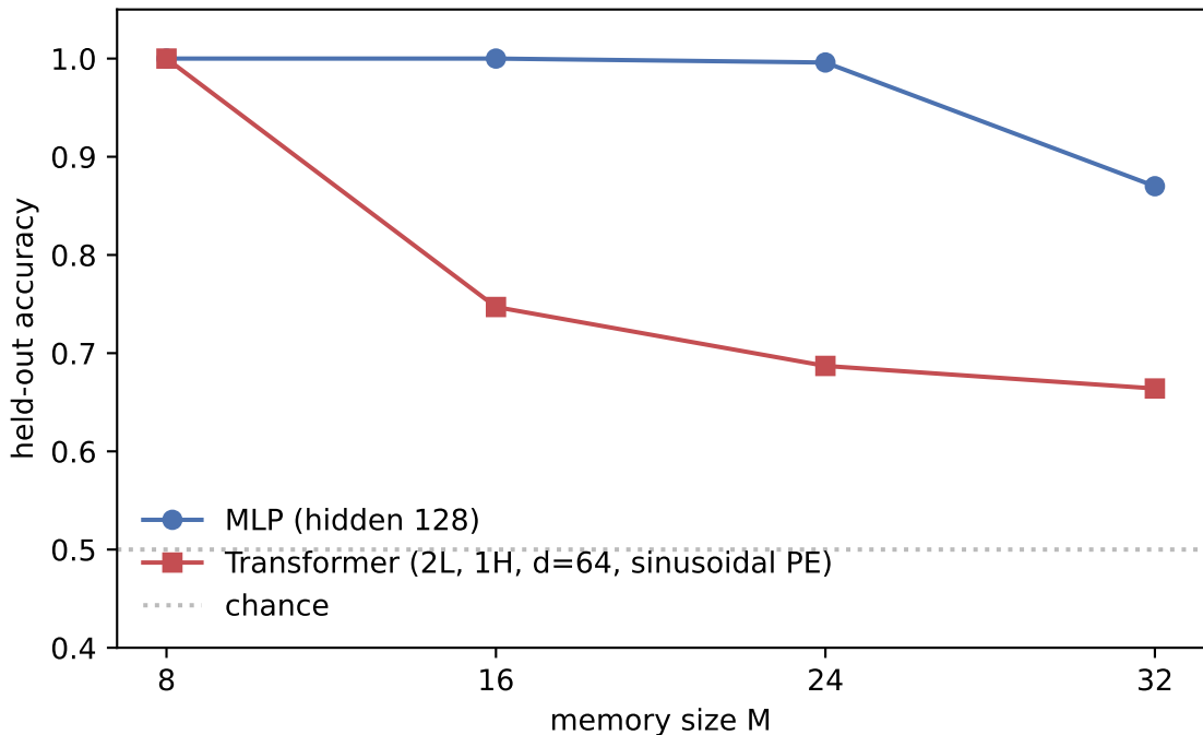
Single-lookup accuracy vs memory size (6000 iters)
