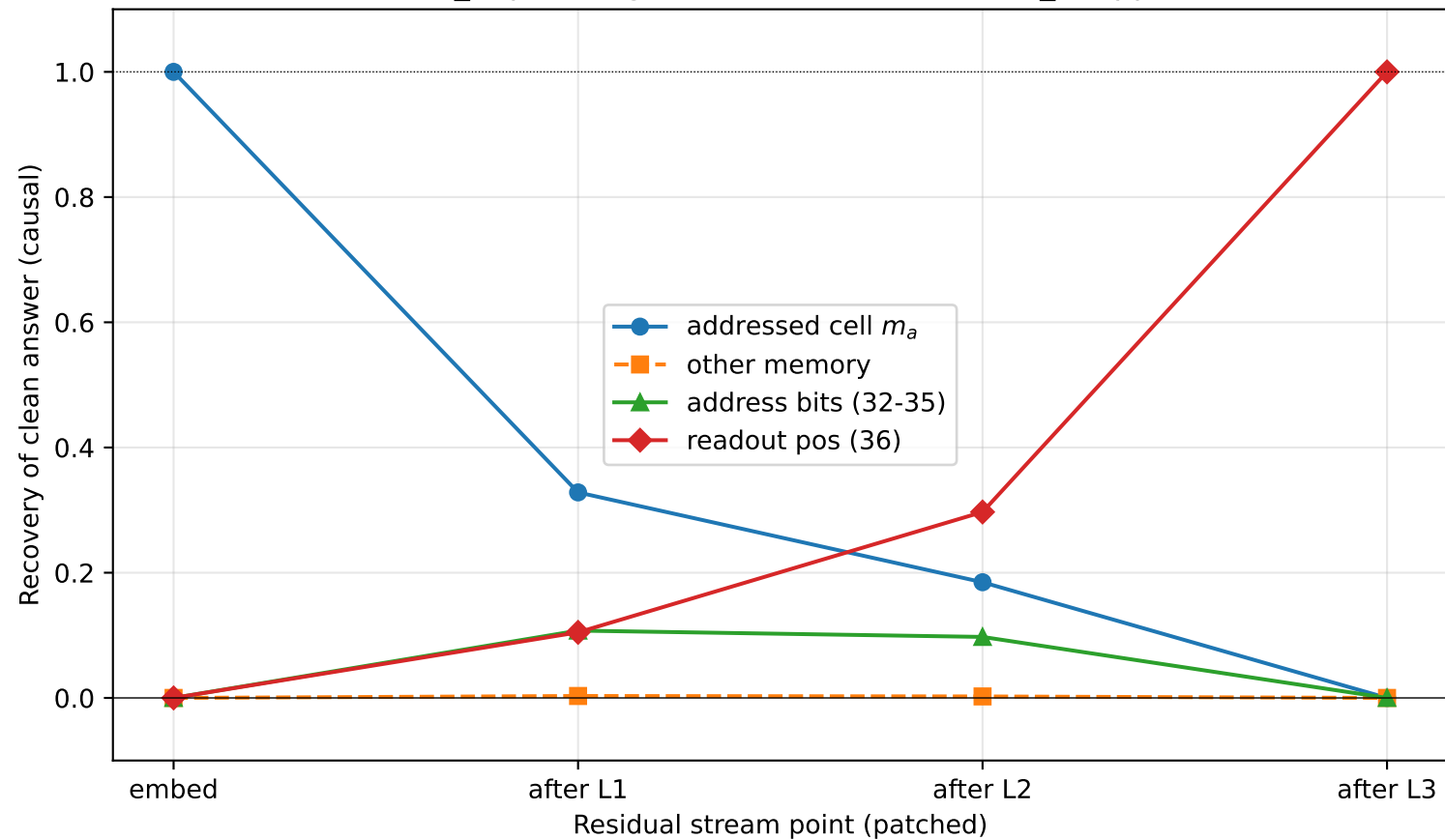
Causal trace of m_a : patching clean residual into the m_a -flipped run ( M=32 )
