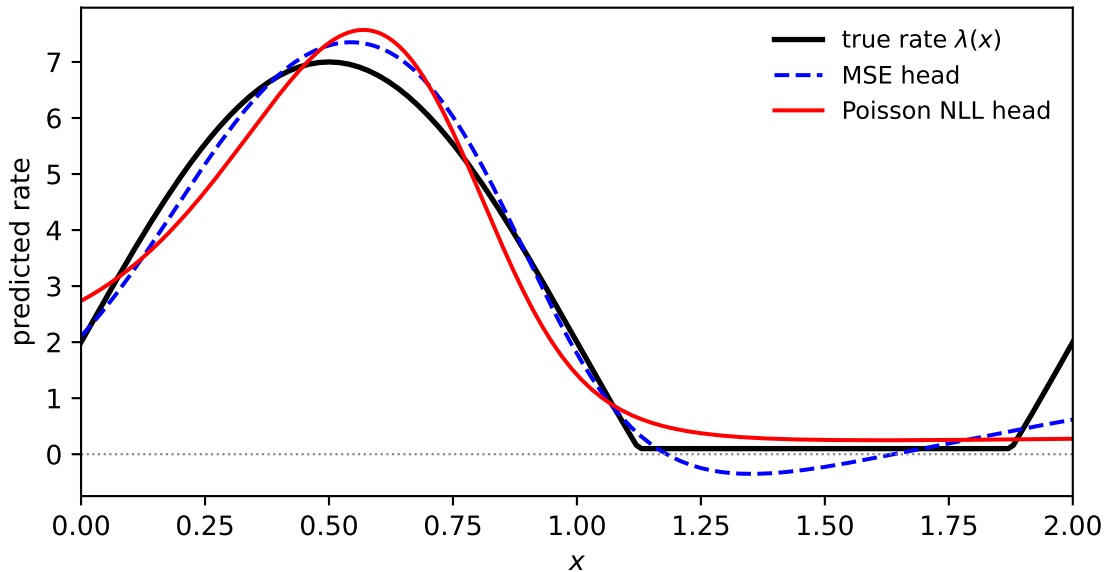
Poisson vs MSE head: count regression
