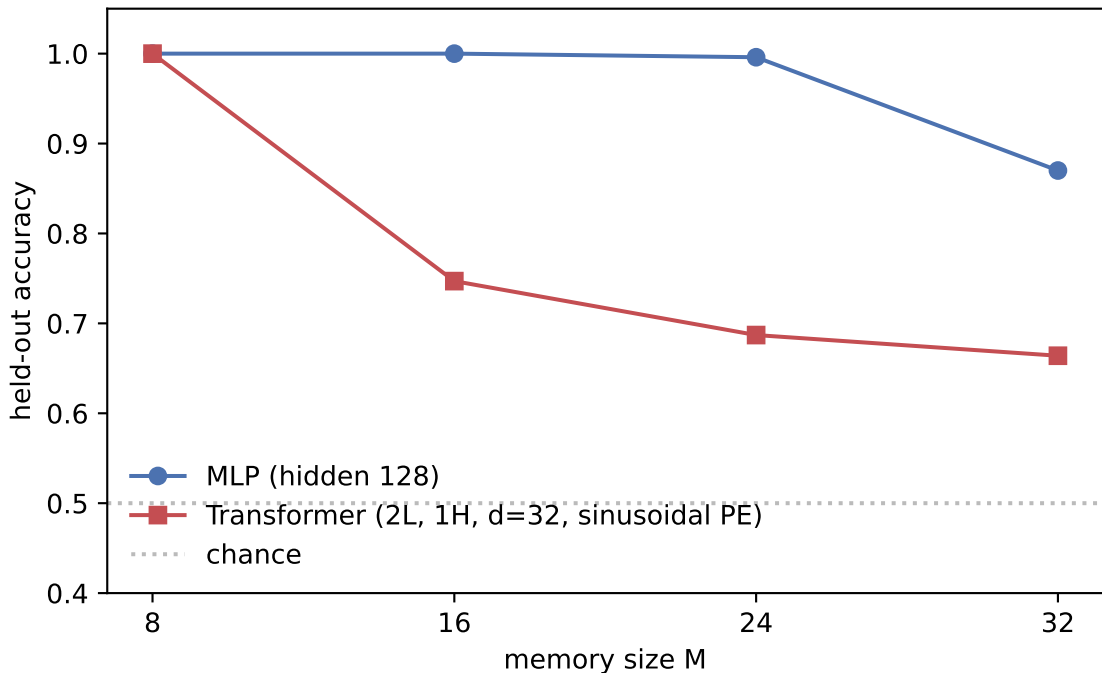
Single-lookup accuracy vs memory size (3000 iters)
