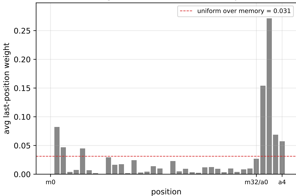
M=32: layer-3 attention (averaged over test set)
