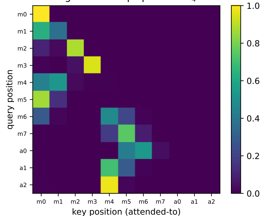
M=8: layer-2 attention (one example, a = 4 )
