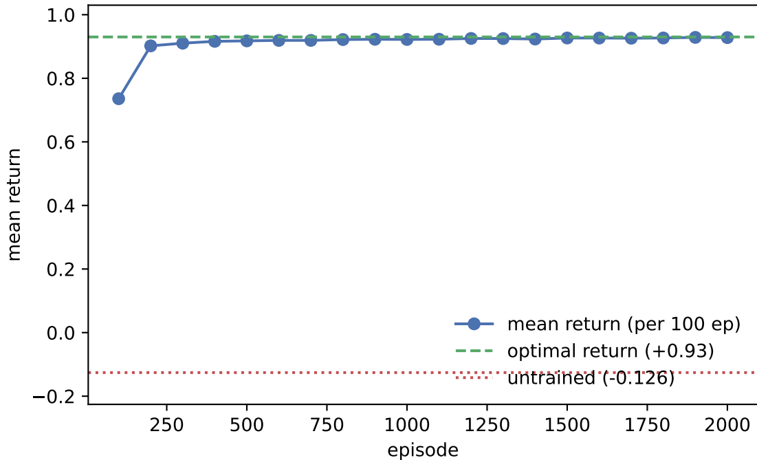
REINFORCE on the 5 \times 5 gridworld (2000 episodes)
