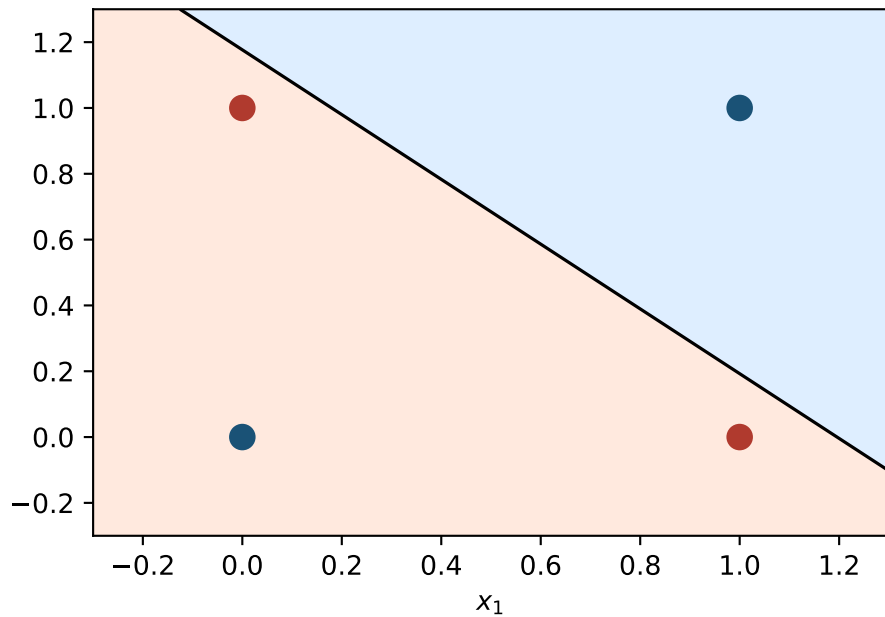
SLP (logistic regression)
