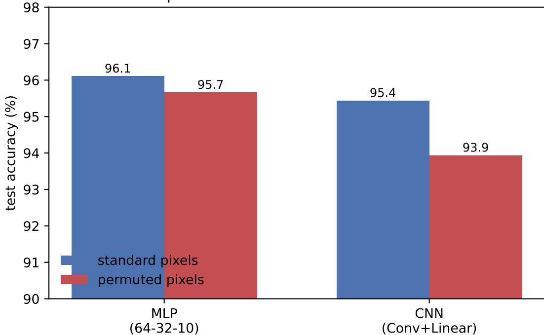
Permuted-pixel control: CNN loses more than the MLP
