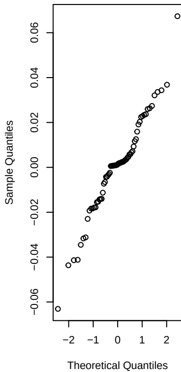
QQ-plot of residuals
