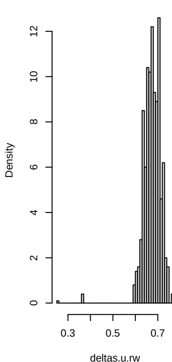
reparameterized random walk
