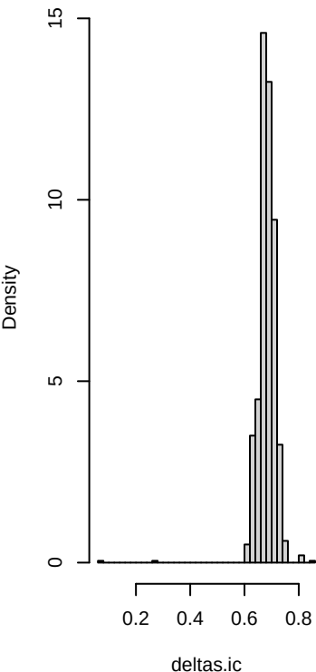
independence chain
