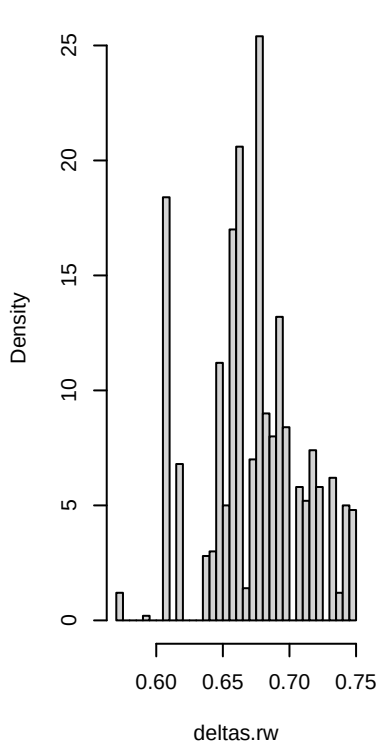
random walk
