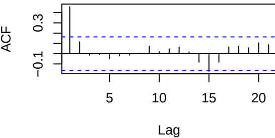
Series Yt.diff
