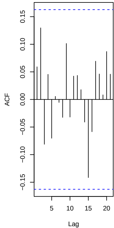
Residuals
