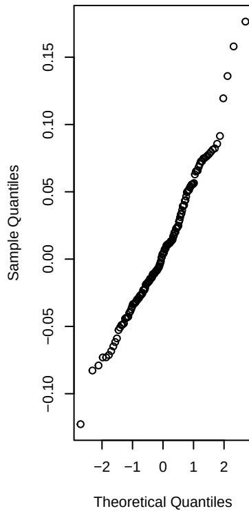
QQ-plot
