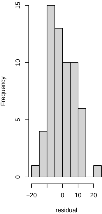
histogram of residuals
