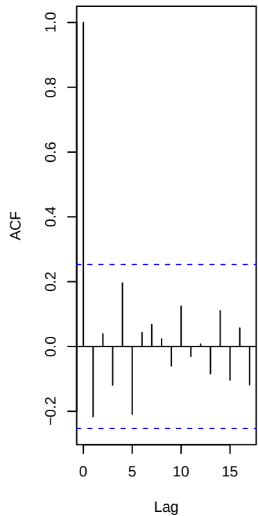
acf of residuals
