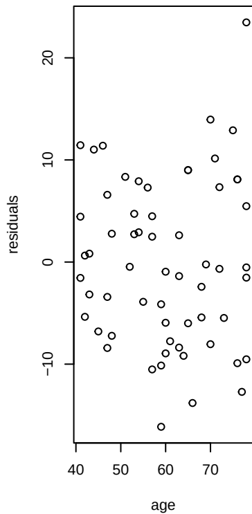
residuals vs age
