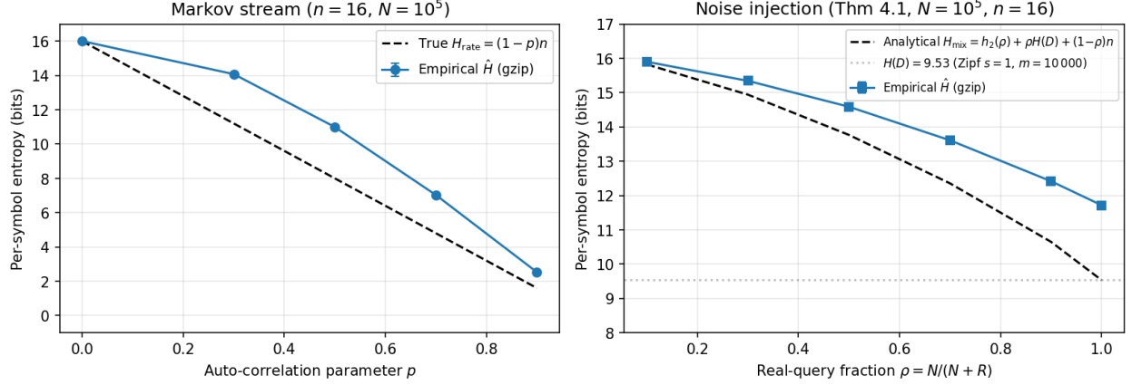
Figure 2: Compression-based entropy estimation against analytically known entropy rates ( n = 16 , N = 10^5 , 5 seeds, error bars \pm 1\sigma ). Left: first-order Markov stream with auto-correlation parameter p , entropy rate H_{\text{rate}} = (1 - p)n . Right: real Zipf queries ( s = 1 , m = 10\,000 ) mixed with uniform filler at fraction \rho , predicted entropy H_{\text{mix}} = h_2(\rho) + \rho H(D) + (1 - \rho)n from Theorem 5.1.
