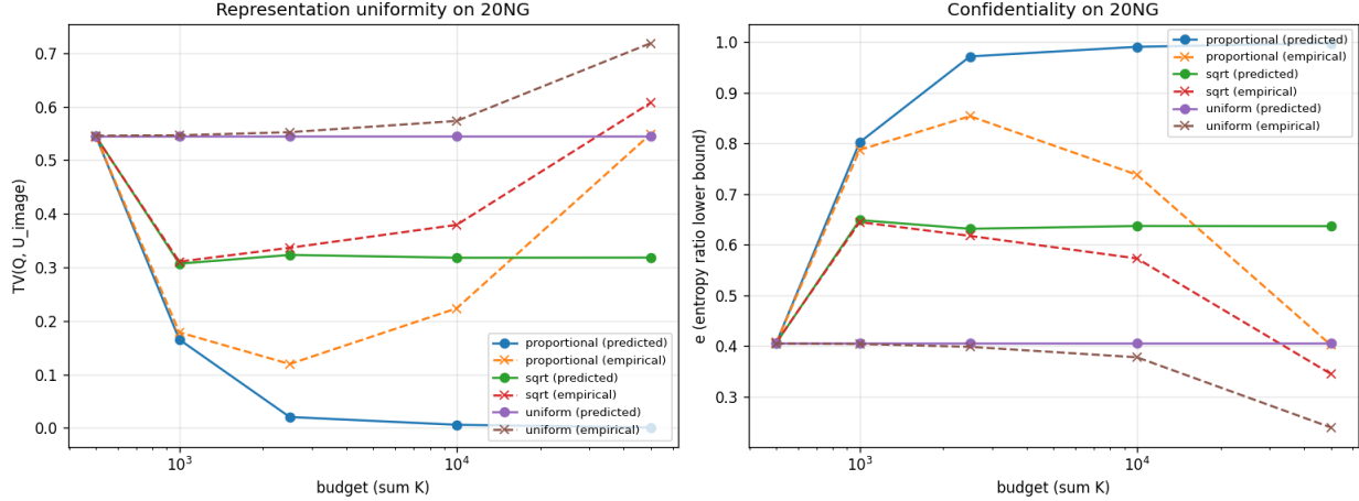
Figure 3: Homophonic encoding on the 20 Newsgroups distribution. Left: representation uniformity d_{TV}(Q, U_{\text{img}}) versus budget for the three allocators (solid: predicted; dashed: empirical at N = 30,000 ). Right: lower bound on the entropy ratio e from the Fannes-Audenaert inequality. Proportional allocation dominates uniform and square-root at every budget.
