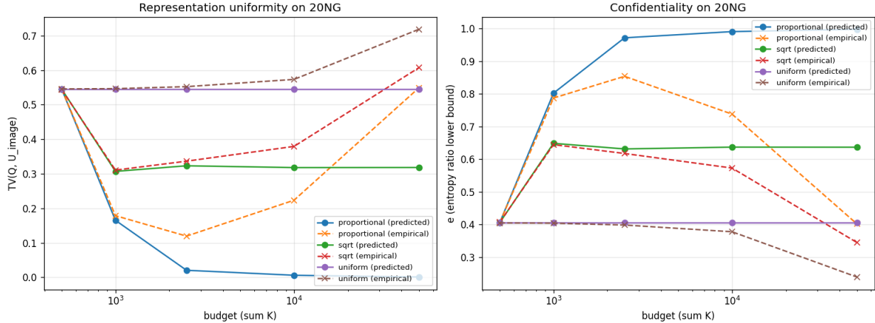
Figure 2: Homophonic encoding on the 20 Newsgroups distribution. Left: representation uniformity d_{TV}(Q, U_{\text{im}}) versus budget for the three allocators (solid: predicted; dashed: empirical at N = 30,000 ). Right: lower bound on the entropy ratio e from the Fannes-Audenaert inequality. Proportional allocation dominates uniform and square-root at every budget.
