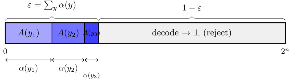
Figure 1: Acceptance predicate partition of the n -bit hash space. Each value y \in Y is assigned an acceptance set A(y) with probability \alpha(y) = |A(y)|/2^n . Under Shannon-optimal allocation \alpha(y) = \varepsilon \cdot p_y (where p_y = \Pr[f(X) = y] ), region widths are proportional to value frequencies: the dominant value y_1 occupies the largest region. A hash falling in A(y) decodes to y ; a hash outside the accepted region (total measure 1 - \varepsilon ) decodes to \perp . The Shannon-frequency duality (§6.2) holds because the same allocation that minimizes the per-element bit cost ( -\log_2 \varepsilon + H(Y) ) also makes the cipher value distribution match the latent value distribution, defeating frequency analysis.
