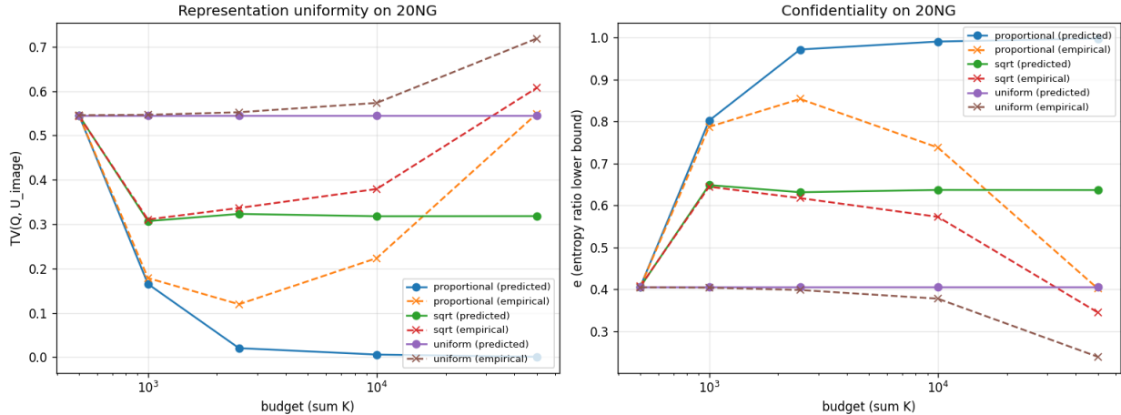
Figure 3: Homophonic encoding on the 20 Newsgroups distribution. Left: representation uniformity d_{TV}(Q, U_{im}) versus budget for the three allocators (solid: predicted; dashed: empirical at N = 30,000 ). Right: lower bound on the entropy ratio e from the Fannes-Audenaert inequality. Proportional allocation dominates uniform and square-root at every budget.
