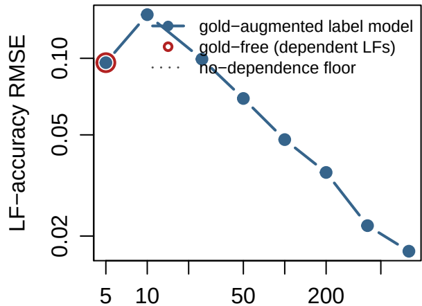
A. Gold restores identifiability (T4)
