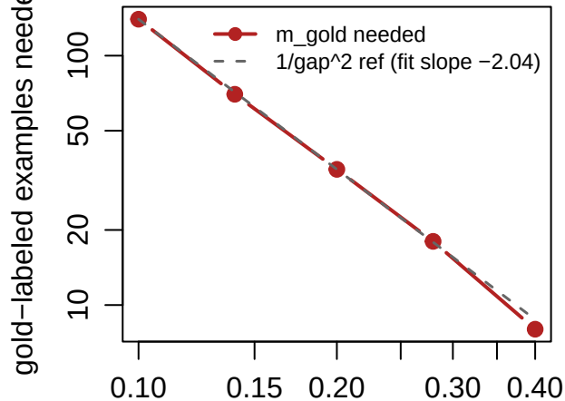
B. Sample complexity scales 1/\text{gap}^2
