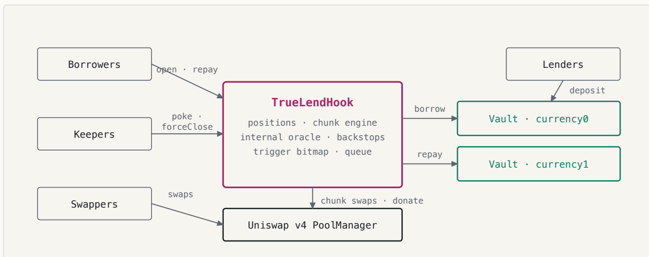
Figure 5. System architecture. One hook instance serves any number of pools; initializing a pool with the hook — an ERC-20 pair or a native-ETH pool, the latter WETH-bridged at the hook boundary — automatically deploys its two vaults and makes it a lending market.
