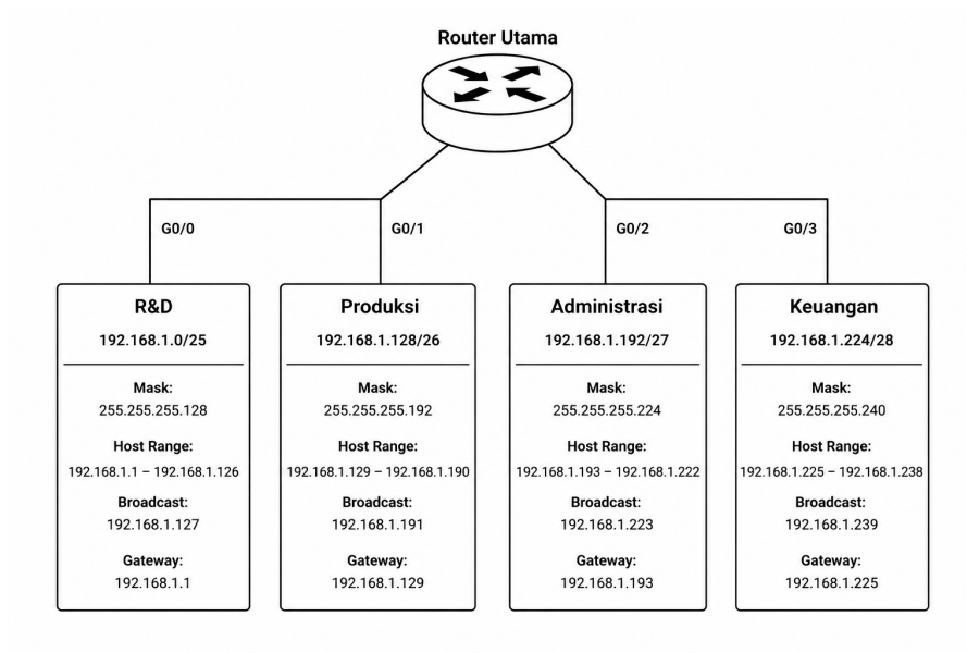
Gambar 2: Topologi star
