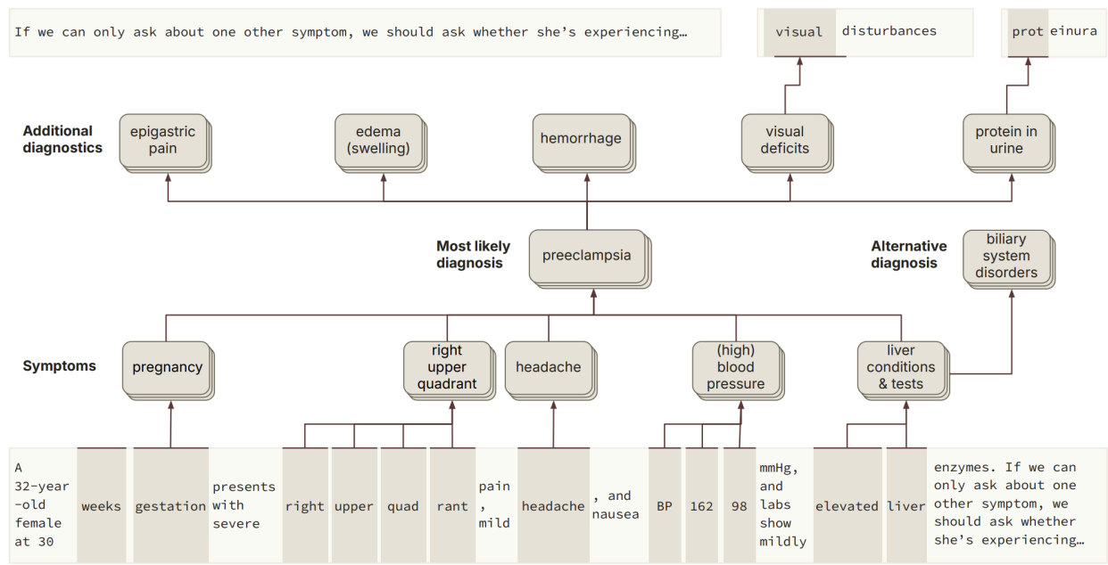
Figure 2. Attribution graph for Claude 3.5 Haiku (Lindsey et al. 2025). Patient-status features activate a preeclampsia feature alongside competing hypotheses ( biliary system disorders ); the preeclampsia feature in turn activates features for confirmatory symptoms, which inform the model’s leading completions: “visual disturbances” and the runner-up, “proteinuria”.
