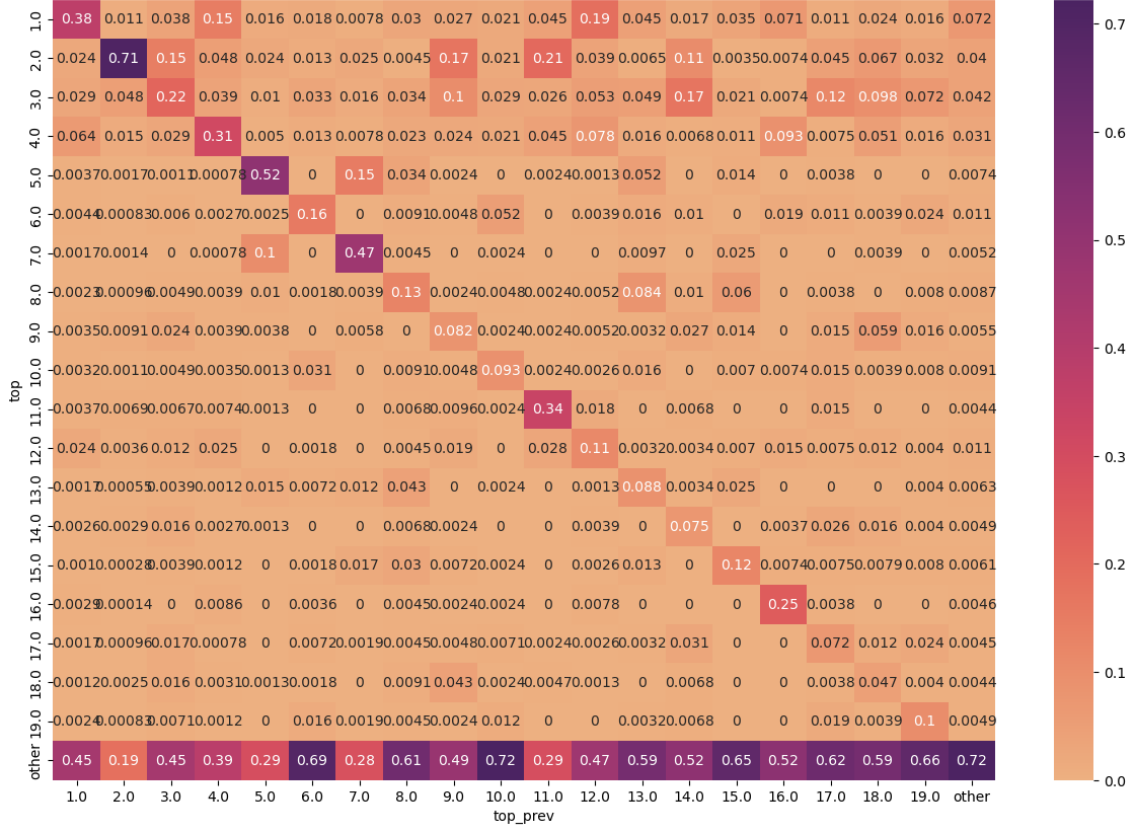
Figure 8: The probability of performing the action sequence s on trial t conditional on the sequence done on the previous trial t-1 : P(s_t|s_{t-1}) . The top 19 sequences are displayed and the remaining thousands are grouped as "other". Sequences are ordered by their frequency of occurrence in the data. Darker colors indicate higher probability. Normalized by sequence (columns).
