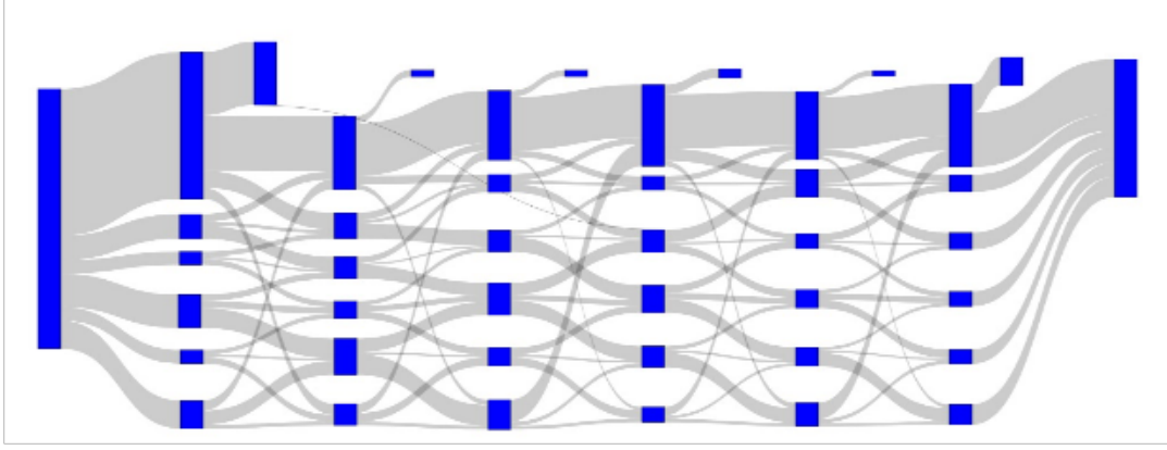
Figure 7: Action transitions in level 1 puzzles in a flattened version of 5. All subjects start on the leftmost node and traverse the plot rightwards. From the initial state, line widths represent the probability of transitions to subsequent nodes and node widths, their occupancy. Rewards are available on the nodes on the top row, growing in value from left to right. The rightmost node represents a reward of 0.
