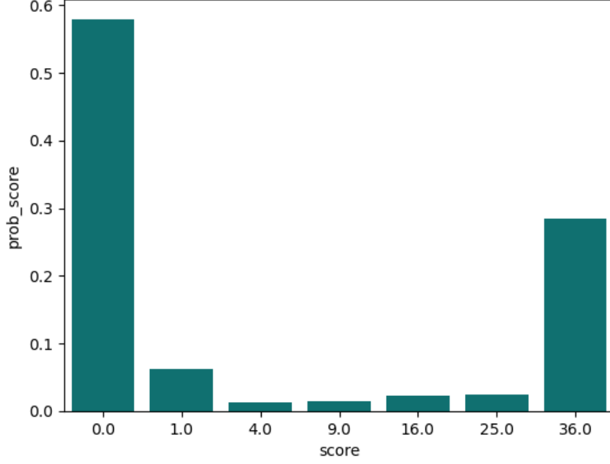
Figure 5: The probability of getting rewards for all possible reward sizes.
